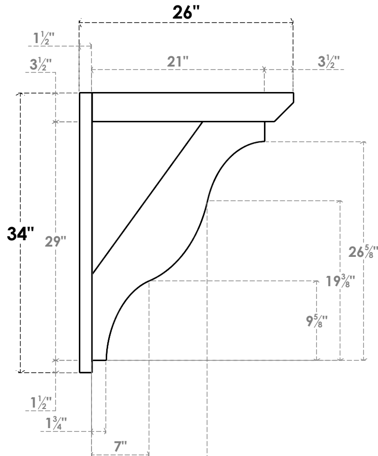
SIDE PROFILE
